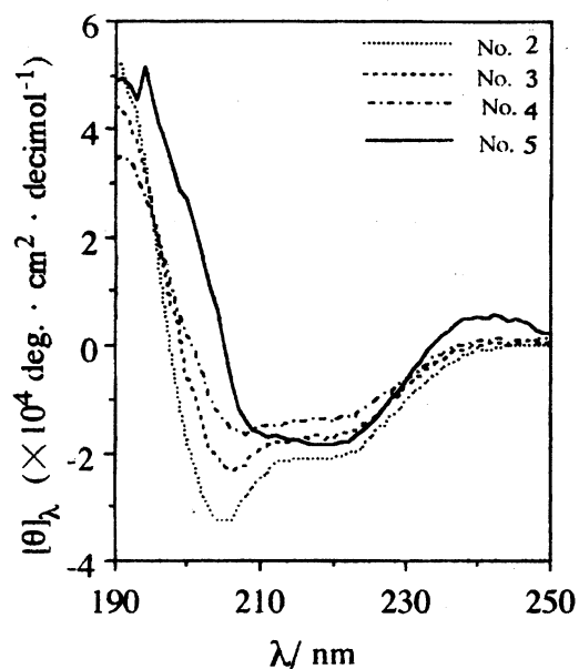
Fig. 4. CD spectra of poly(Trp(Form)-co-Ala) in HFIP.
